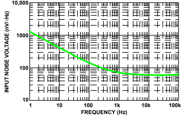
FIGURE 23. SIMULATED INPUT NOISE VOLTAGE
